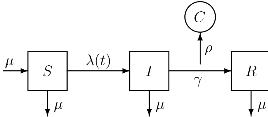
FIGURE 7. Diagram of the SIR model. The host population is divided into three classes according to their infection status: S, susceptible hosts; I, infected (and infectious) hosts; R, recovered and immune hosts. Births result in new susceptibles and all individuals have a common death rate \mu . Since the birth rate equals the death rate, the expected population size, N = S + I + R , remains constant. The S→I rate, \lambda , called the force of infection , depends on the number of infectious individuals according to \lambda(t) = \beta I/N . The I→R, or recovery, rate is \gamma . The case reports, C , result from a process by which infections are recorded with probability \rho . Since diagnosed cases are treated with bed-rest and hence removed, infections are counted upon transition to R.
